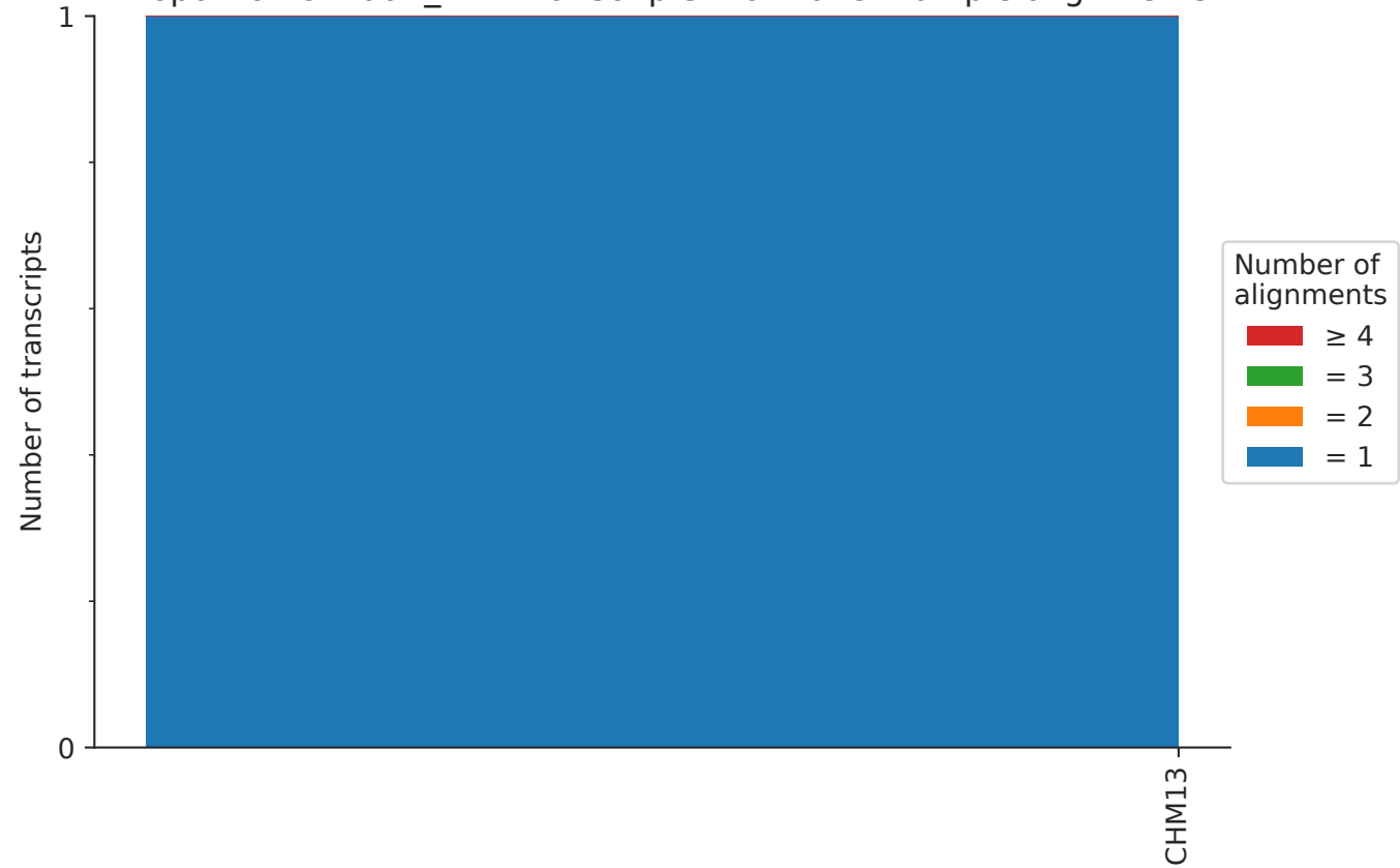
Proportion of vault_RNA transcripts that have multiple alignments
