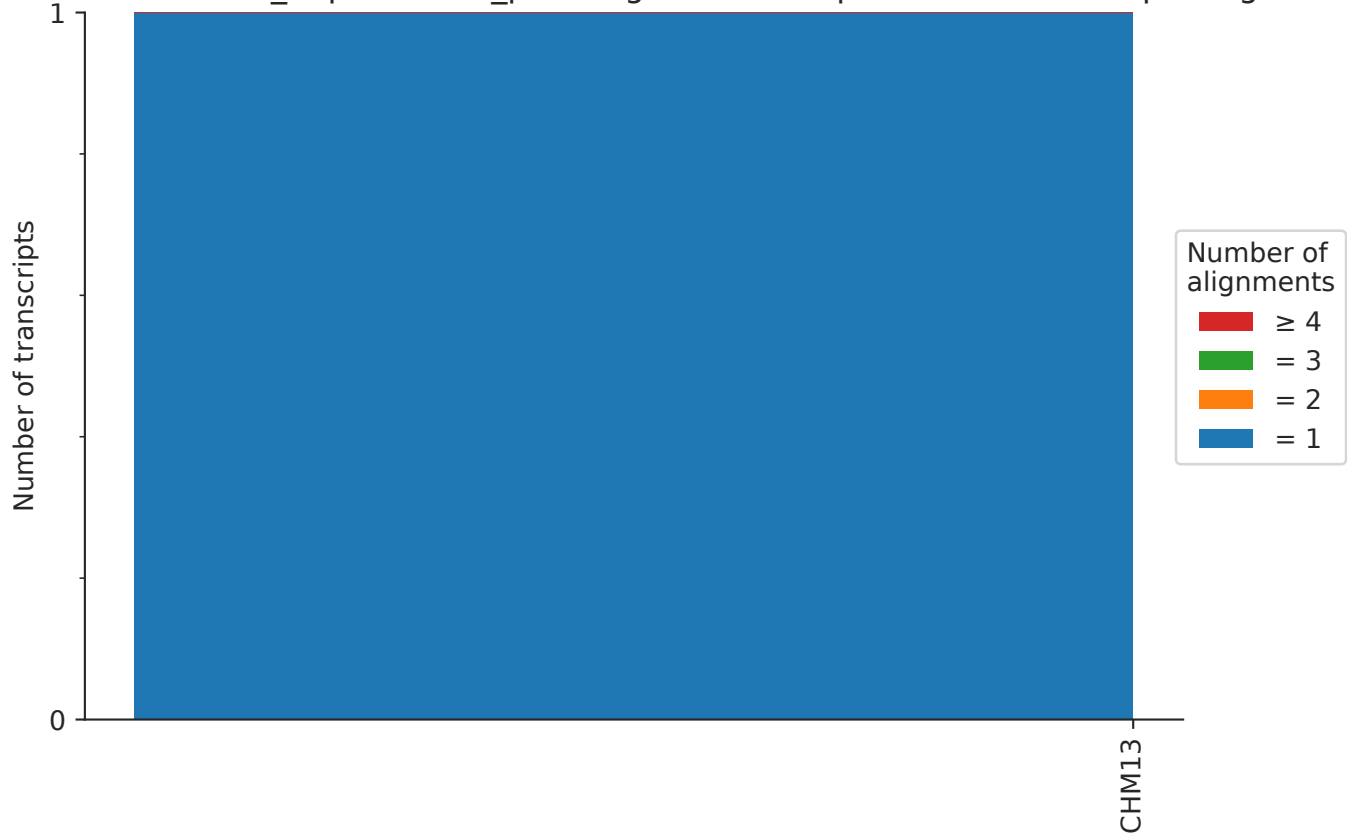
Proportion of translated_unprocessed_pseudogene transcripts that have multiple alignments
