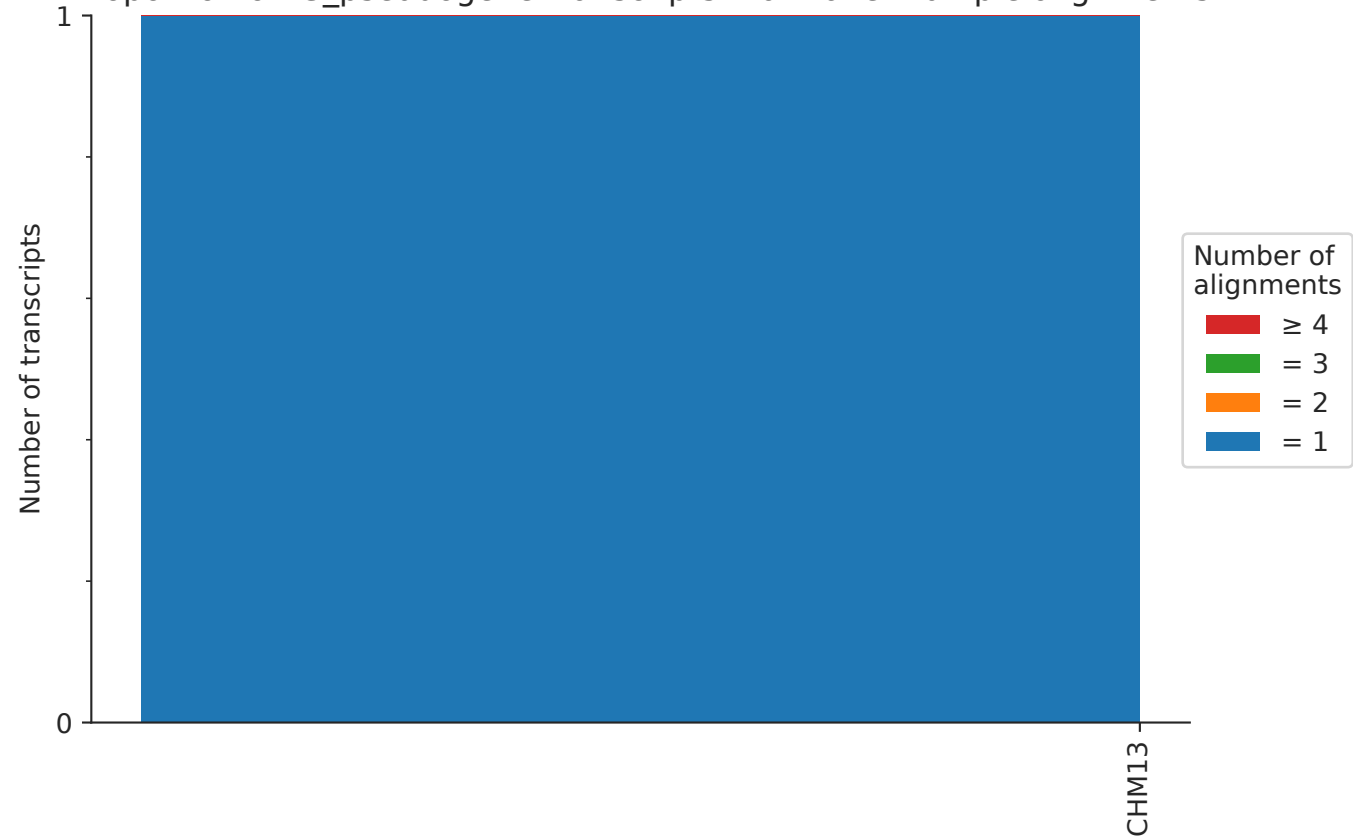
Proportion of IG_pseudogene transcripts that have multiple alignments
